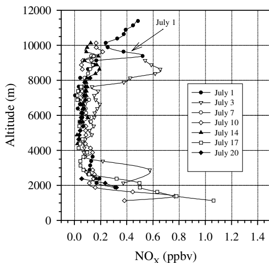
Figure 5. Observed vertical \text{NO}_x distribution (in ppbv) on single EULINOX mission days indicated by different symbols (single cloud penetrations excluded).
