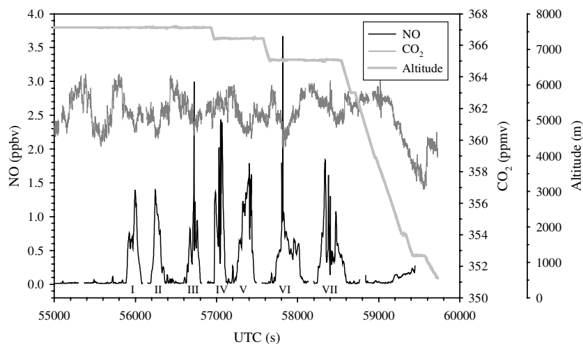
Figure 14. Mixing ratio of NO (black line) and CO 2 (dark gray line), and altitude (light gray line) versus time from the flight of 17 July. Seven penetrations of a squall line at different altitudes are labeled I–VII.
