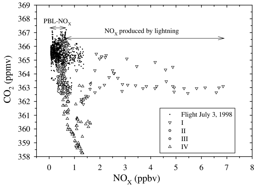
Figure 13. Data of CO 2 versus NO x mixing ratios for the flight from 3 July. Convective clouds with lightning (labeled I + IV) and without lightning (labeled II + III) were penetrated. Arrows indicate the ranges of data obtained in clouds from transported PBL NO x and from lightning-produced NO x .
