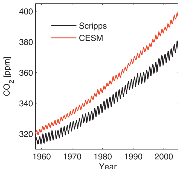
FIG. 2. Observed atmospheric \text{CO}_2 at Mauna Loa (black) compared to \text{CO}_2 in CESM sampled at Mauna Loa (red). The growth rate is higher in CESM than observed; the annual mean difference of 4 ppm in 1958 grows to 20 ppm by 2005. The observations shown are from the SIO carbon program (Keeling et al. 2001).
