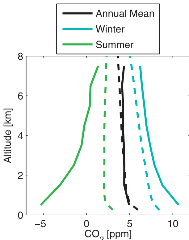
FIG. 12. Vertical profiles in NOAA GMD aircraft data (solid lines) and CESM (dashed lines). We plot annual mean, winter (January–March) and summer (July–September) for sites between 40° and 60°N. This figure follows an approach similar to Stephens et al. (2007), with the mole fractions recentered by the deseasonalized surface mole fraction at South Pole.
