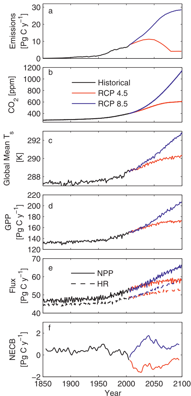
FIG. 15. Differences between the CESM RCP4.5 and RCP8.5 twenty-first-century scenarios: (a) annual mean global emissions for the historical simulation (1850–2005) (black) and for RCP4.5 (red) and RCP8.5 (blue) between 2005 and 2100; (b) monthly mean atmospheric \text{CO}_2 sampled at Mauna Loa; (c) resulting global mean surface temperatures; (d) globally integrated and annually averaged gross primary production (GPP); (e) net terrestrial biospheric fluxes as net primary production (solid) and heterotrophic respiration (dashed). (f) Net ecosystem carbon balance (NECB) smoothed using a 10-yr filter, which represents the net land-to-atmosphere flux of \text{CO}_2 in CESM including harvest, fire, and land use change.
