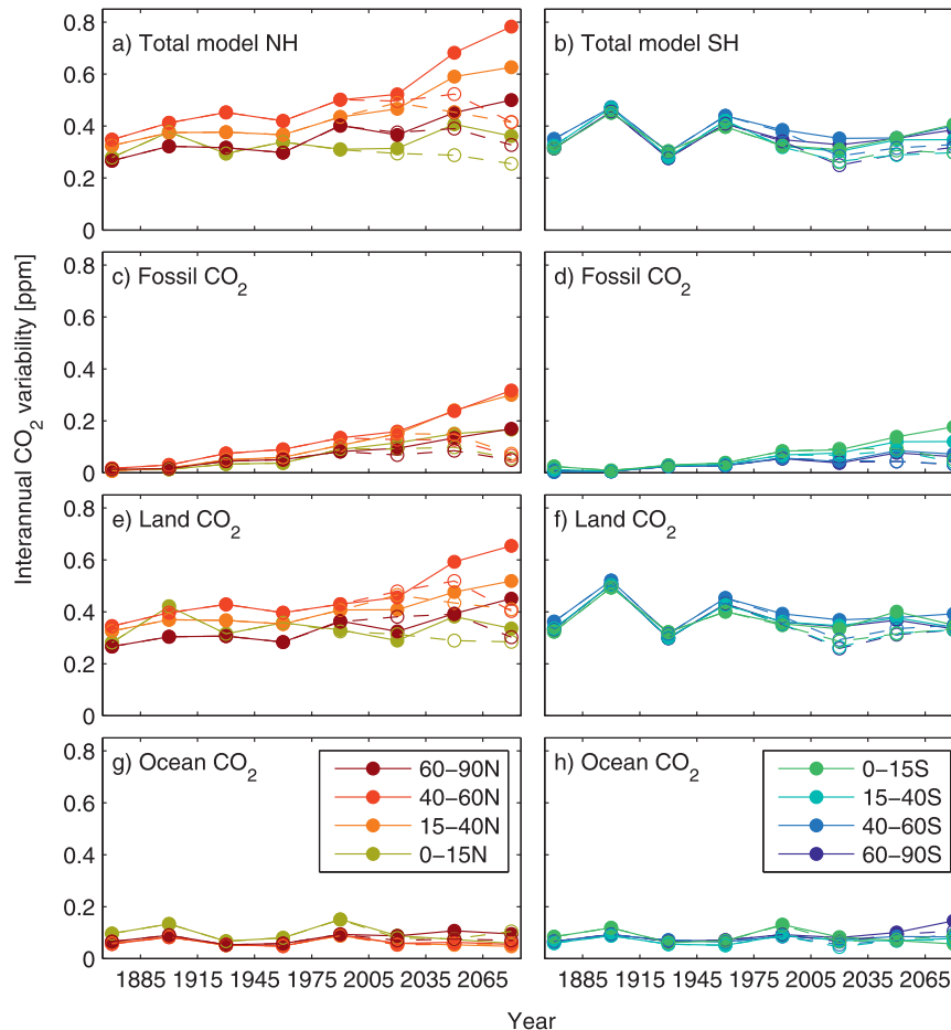
FIG. 14. Interannual variability (IAV) in surface CESM \text{CO}_2 for eight latitude bands in the (left) Northern Hemisphere and (right) Southern Hemisphere: (a),(b) IAV for the total \text{CO}_2 in CESM, (c),(d) IAV for the fossil \text{CO}_2 component, (e),(f) IAV for the land component of \text{CO}_2 , and (g),(h) IAV for the ocean component of \text{CO}_2 . The solid symbols show IAV from RCP8.5 and the open symbols show IAV from RCP4.5.
