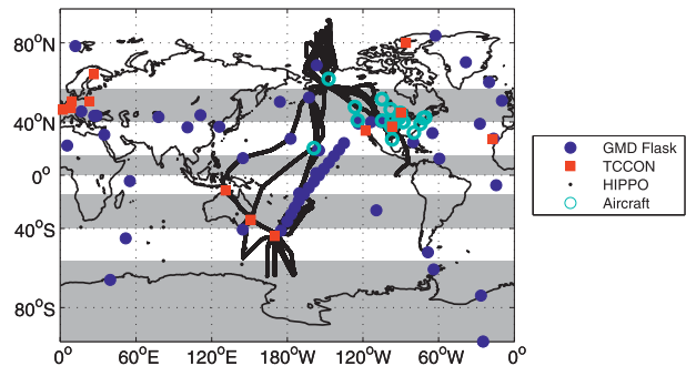
FIG. 1. Locations of observations used in this paper: CESM at Global Monitoring Division (GMD) flask sites (blue circles), TCCON observatories (red squares), NOAA aircraft profile locations (cyan circles), and along HIPPO flight tracks (black dots). The alternating zonal color bands demark the regions used for averaging the data: 60^\circ\text{--}90^\circ\text{S} , 40^\circ\text{--}60^\circ\text{S} , 15^\circ\text{--}40^\circ\text{S} , 0^\circ\text{--}15^\circ\text{S} , 0^\circ\text{--}15^\circ\text{N} , 15^\circ\text{--}40^\circ\text{N} , 40^\circ\text{--}60^\circ\text{N} , and 60^\circ\text{--}90^\circ\text{N} .
