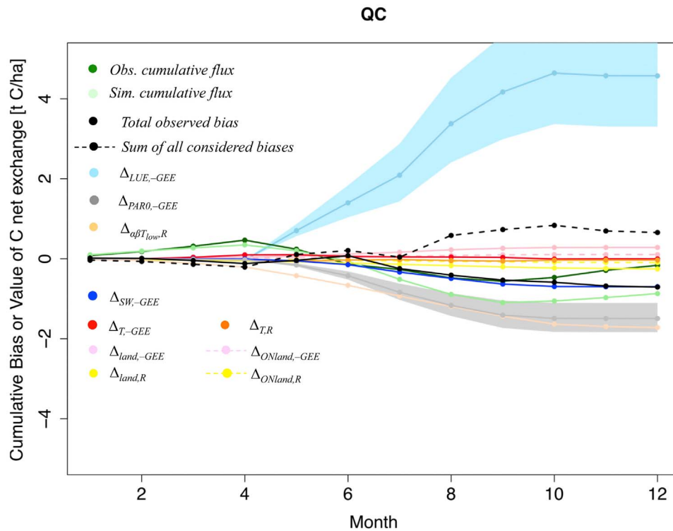
Figure 10. Cumulative biases in NEE (F_{sim} - F_{obs}) in 2004 at QC and the contributions from different error sources. The values indicated at the end of the year quantify the net impact of a bias in a particular variable on the simulated annual carbon balance. \Delta_{ONland,-GEE} and \Delta_{ONland,R} have also been introduced to indicate the smaller biases that would result from adopting a higher-resolution land cover product like the Ontario Land Cover data set, with its reported error of 10%. Here \Delta_{\alpha\beta T_{low},R} is an aggregate bias resulting from assuming the incorrect relationship between T and R (Figure 7). The observed (dark green) and simulated (light green) cumulative carbon fluxes are also shown, along with the total bias (black), which is the difference between observed and simulated carbon fluxes. The sum of all biases considered in this study is shown as the dashed black line. The shaded regions for \Delta_{LUE,-GEE} and \Delta_{PAR_0,-GEE} reflect the ranges in biases stemming from uncertainties in the fits to eddy covariance fluxes to determine “observed” PAR_0 and LUE and the negative correlations between the two parameters. See section 6.6.2 for explanation.
