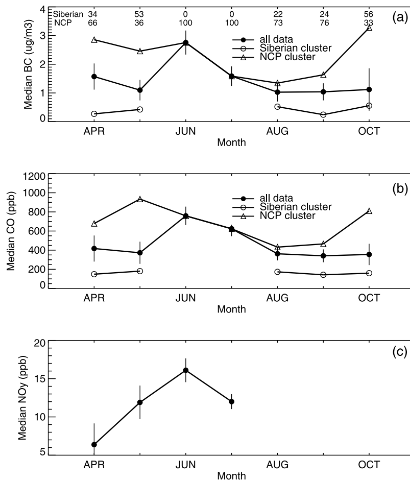
Figure 4. Monthly variations of daytime (0800–1800 LT) (a) BC, (b) CO, and (c) NO y at the Miyun site from April to October 2010. The NO y data were not available since late July because of the instrument failure. Median concentrations of BC and CO of the Siberian and the NCP air mass groups discussed in section 4.3 were also given. The numbers at the top of 4a are the percentages (%) of the Siberian and the NCP air masses in each month. The error bars are 1/4 of the standard deviations.
