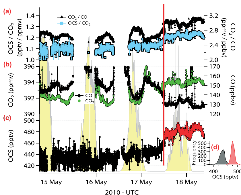
Figure 7. A change of airmass on 17 May (red line) led to (a) an increase in the CO 2 /CO ratio (black) and OCS/CO 2 ratio (blue), (b) a decrease in CO (black) and increase in minimum CO 2 (green), and (c) an increase in OCS of 50 pptv. (d) Histogram of OCS data before (black, 15–17 May) and after (red, 17–19 May) shows the increase in mixing ratio (from 436 to 480 pptv) and the reduction in variability of OCS (11 pptv to 7 pptv) evident after the airmass change.
