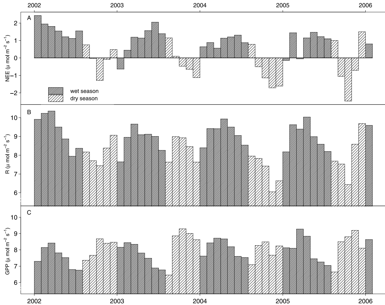
Figure 5. Monthly time series (49 months) of (a) net ecosystem exchange of CO 2 (NEE, \mu\text{mol m}^{-2} \text{s}^{-1} ), (b) ecosystem respiration (R, \mu\text{mol m}^{-2} \text{s}^{-1} ), and (c) gross primary production (GPP, \mu\text{mol m}^{-2} \text{s}^{-1} ). The shading patterns within the bars indicate the season.
