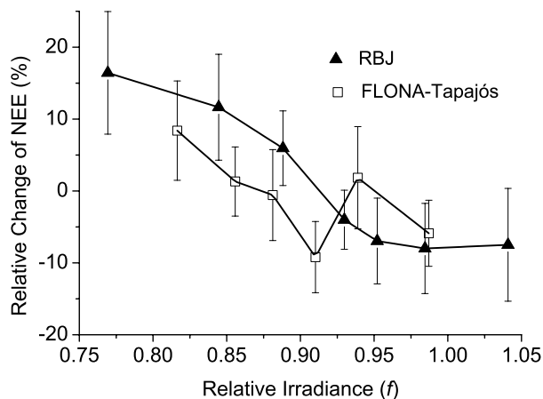
Fig. 9. Relative change of NEE (%NEE) due to biomass burning aerosol loading: calculations for solar zenithal angle ( \alpha ) between 20° and 30°.
