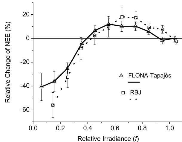
Fig. 6. Relative change of NEE (%NEE) as a function of the relative irradiance ( f ), averaged for all solar zenithal angle intervals ( \alpha ) (from 10^\circ to 70^\circ ). Note that this plot includes clouds and aerosol effects.
