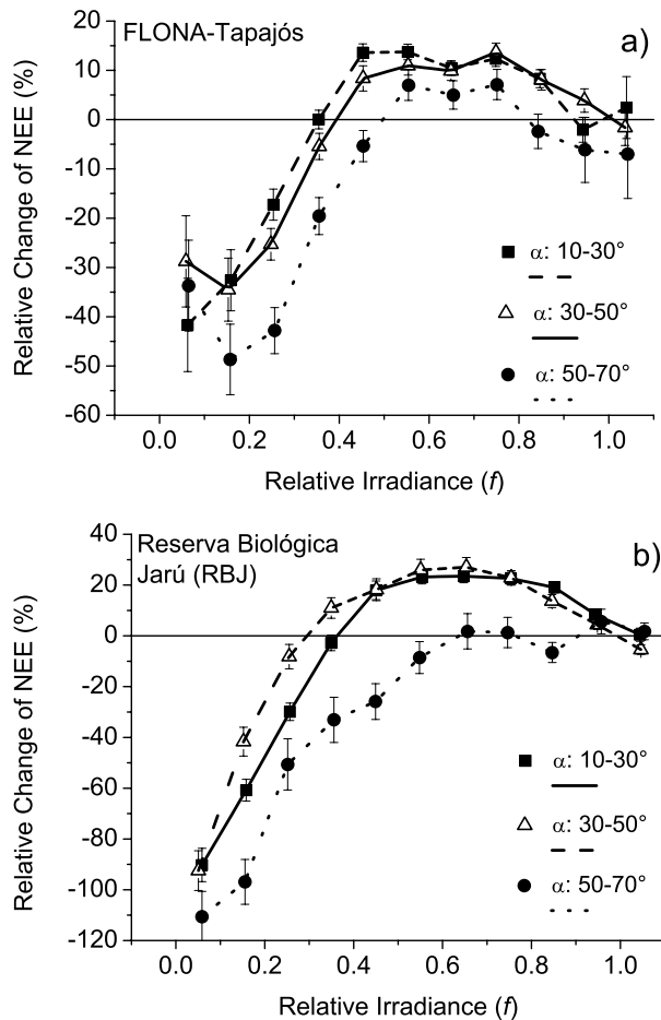
Fig. 5. Relative change of NEE (%NEE) as a function of the relative irradiance ( f ) for three ranges of solar zenithal angle interval ( \alpha ) for the FLONA-Tapajós (a) and RBJ (b) sites.
