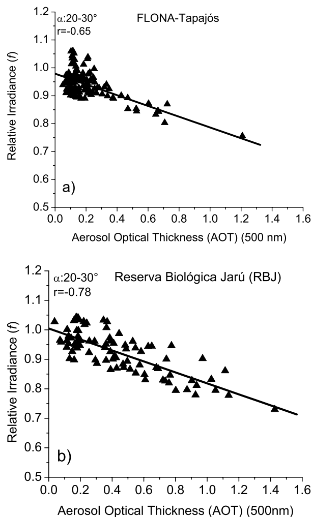
Fig. 7. Relative irradiance ( f ) as a function of AOT at the FLONA-Tapajós (a) and RBJ (b) sites, for solar zenithal angle ( \alpha ) between 20° and 30°. The regressions are statistically significant.
