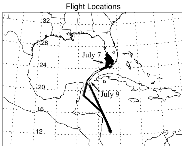
Figure 1. Flight tracks of the WB-57F for 7 and 9 July 2002. The white center of the track indicates the regions where the plumes of CO, NO y , and biomass burning particles were measured.
