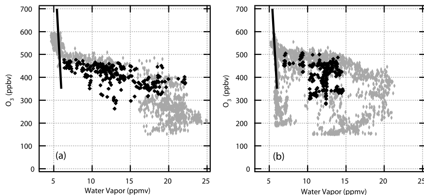
Figure 10. Correlations of ozone and water vapor for the flights of (left) 7 July and (right) 9 July 2002. Shading is the same as in Figure 5.
