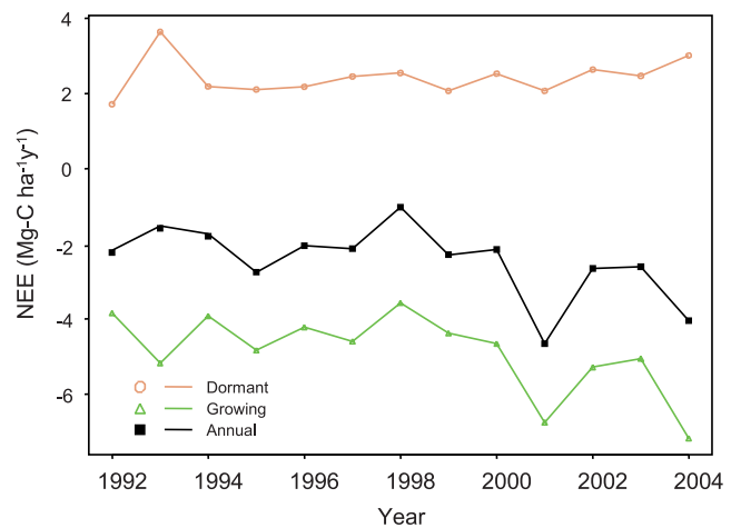
Figure 3. Annual sums of NEE for 1992–2004 (black line with squares) are compared to sums of NEE over the dormant (brown line with circles) and growing season (green line with triangles). Annual sums are calculated for “ecological years,” starting on 28 October which corresponds to the ecosystem transition from carbon uptake to release after the leaves have fallen. Dormant season is 28 October to 15 April and growing season is 15 April to 27 October. The annual trends and anomalies are most closely matched by the growing season NEE sums.
