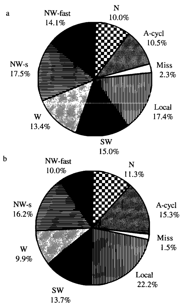
Figure 2. Relative frequency of occurrence of transport patterns at Harvard Forest during (a) the cold season (October–March) and (b) the warm season (April–September).
