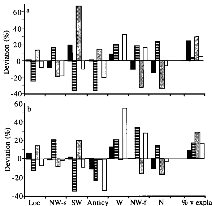
Figure 7. Deviations of mean mixing ratios within each PATH from seasonal mean air temperature (solid column), photosynthetically active radiation (striped column), water-vapor mixing ratio (shaded column), and mixed-layer depth (open column) for (a) winter (December-February) and (b) summer (June-August).
