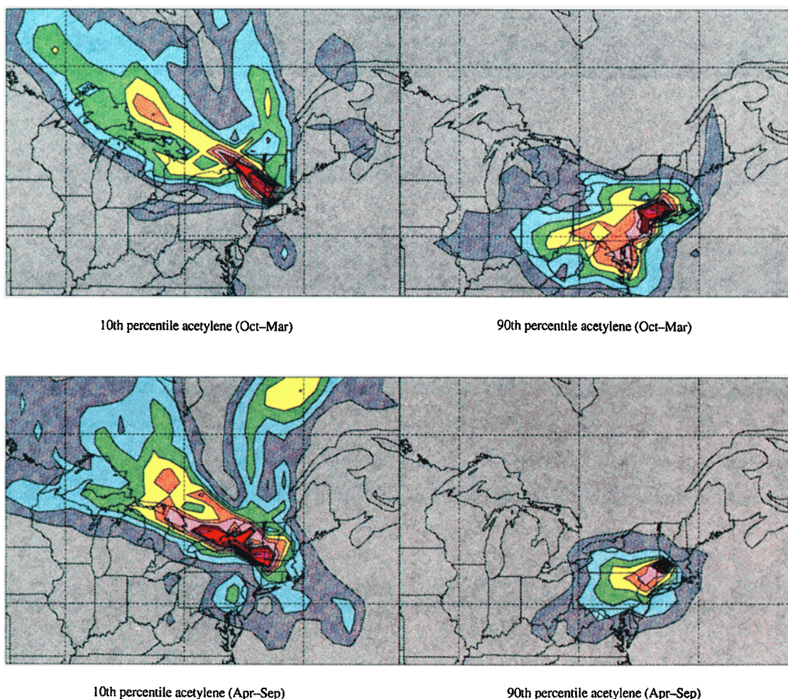
Plate 2. Probability plots showing the likelihood of transport from upwind regions using trajectories that correspond to the lowest 10% and the highest 90% of the acetylene mixing ratios in each season.
