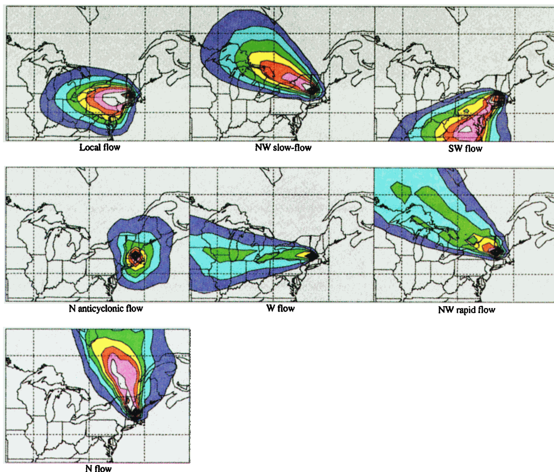
Plate 1. PATH model results depicting seven different flow patterns. Relative probability is contoured; it represents the likelihood of trajectories having crossed the underlying regions. Ten probability intervals are contoured; warmer colors show higher probability.
