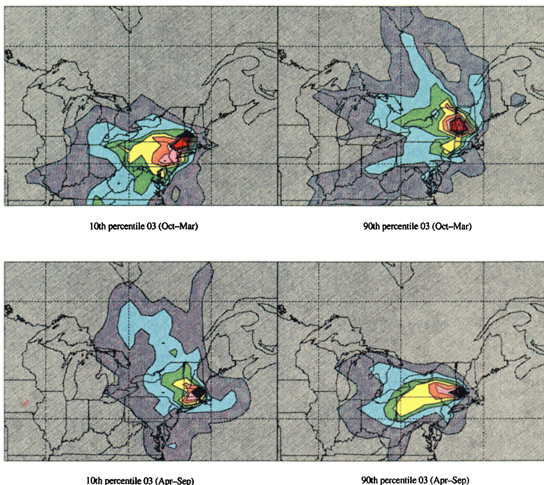
Plate 3. Probability plots showing the likelihood of transport from upwind regions using trajectories that correspond to the lowest 10% and the highest 90% of the ozone mixing ratios in each season.
