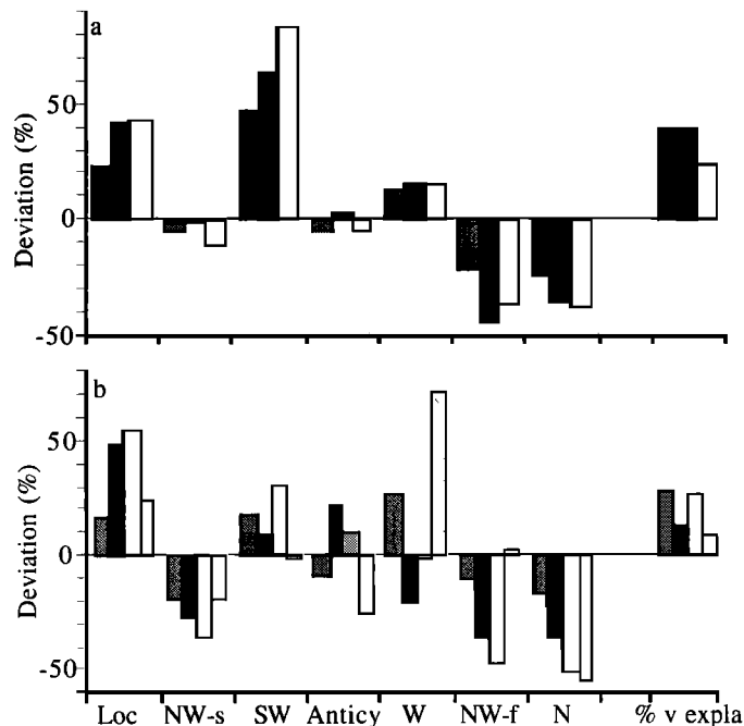
Figure 6. Deviations of mean mixing ratios within each PATH from the seasonal mean mixing ratio of ethane (dark gray column), ethene (solid column), butane (open column), and isoprene (light gray column) for (a) winter (December-February) and (b) summer (June-August). Isoprene was undetectable during winter.
