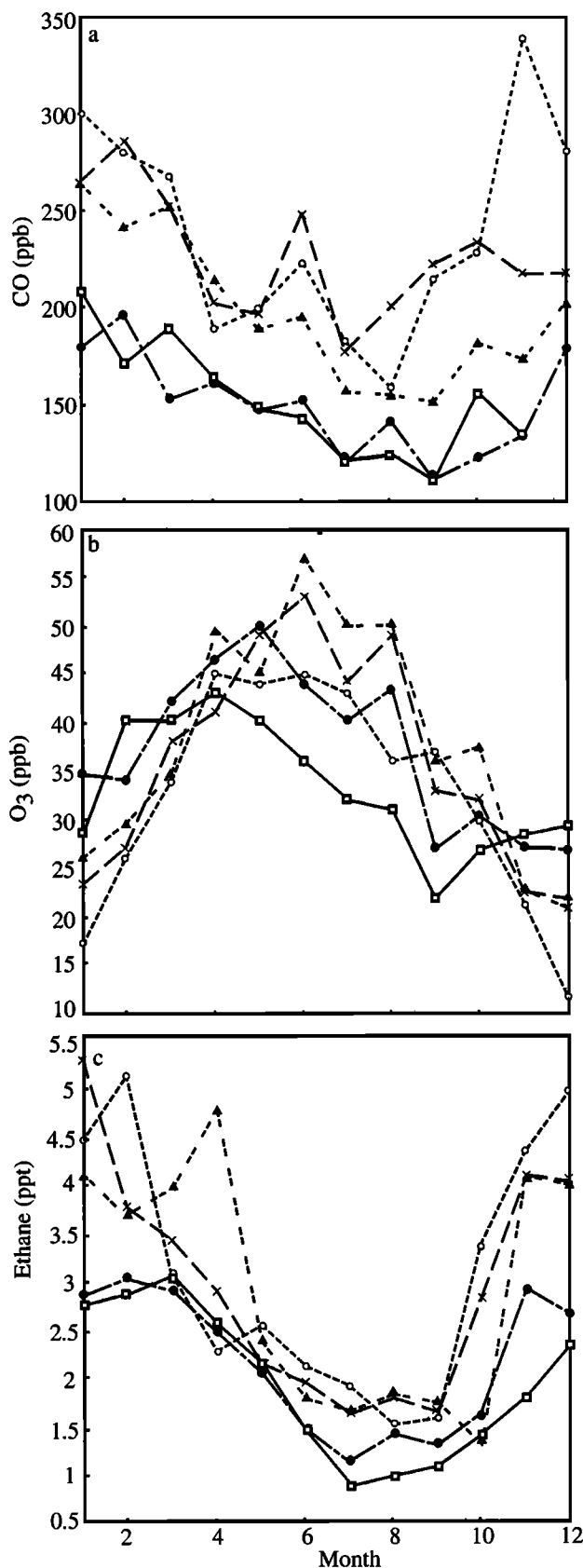
Figure 4. Monthly median mixing ratios showing seasonal signals for (a) CO, (b) O 3 , and (c) ethane under different PATHs (x, Local; open circle, SW; closed triangle, W; closed circle, NW-fast; and open square, N).
