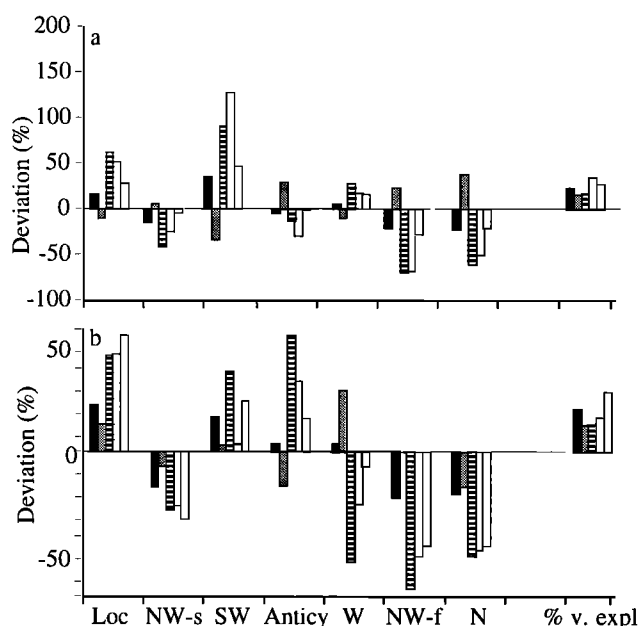
Figure 5. Deviations of mean mixing ratios within each PATH from the seasonal mean mixing ratio of CO (solid column), O_3 (dark gray column), acetylene (striped column), NO_y (light gray column), and NO_x (open column) for (a) winter (December-February) and (b) summer (June-August).
