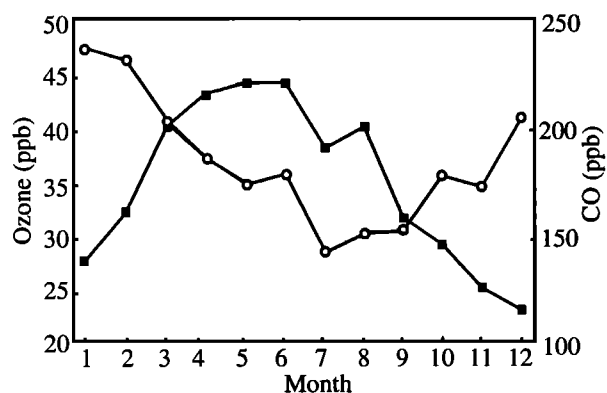
Figure 3. Monthly median mixing ratios showing seasonal signals for O 3 (solid squares) and CO (open circles).
