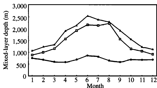
Figure 1. Seasonal and temporal variations by time of day (solid circle, 0700 EST; open square, 1100 EST; solid triangle, 1500 EST) in the monthly average mixed-layer depth at Harvard Forest as calculated by the National Meteorological Center Nested Grid Model.
