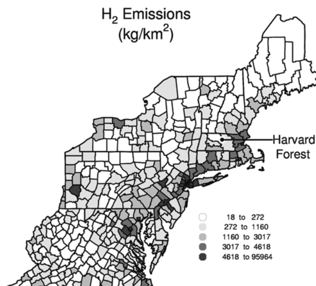
Figure 5. County-level map of the Northeast for hydrogen fossil fuel emissions in kg/area. These values are for the year 1996 and are based on the EPA inventory of CO emissions and 1998 county population and area statistics of the U.S. Census Bureau.
