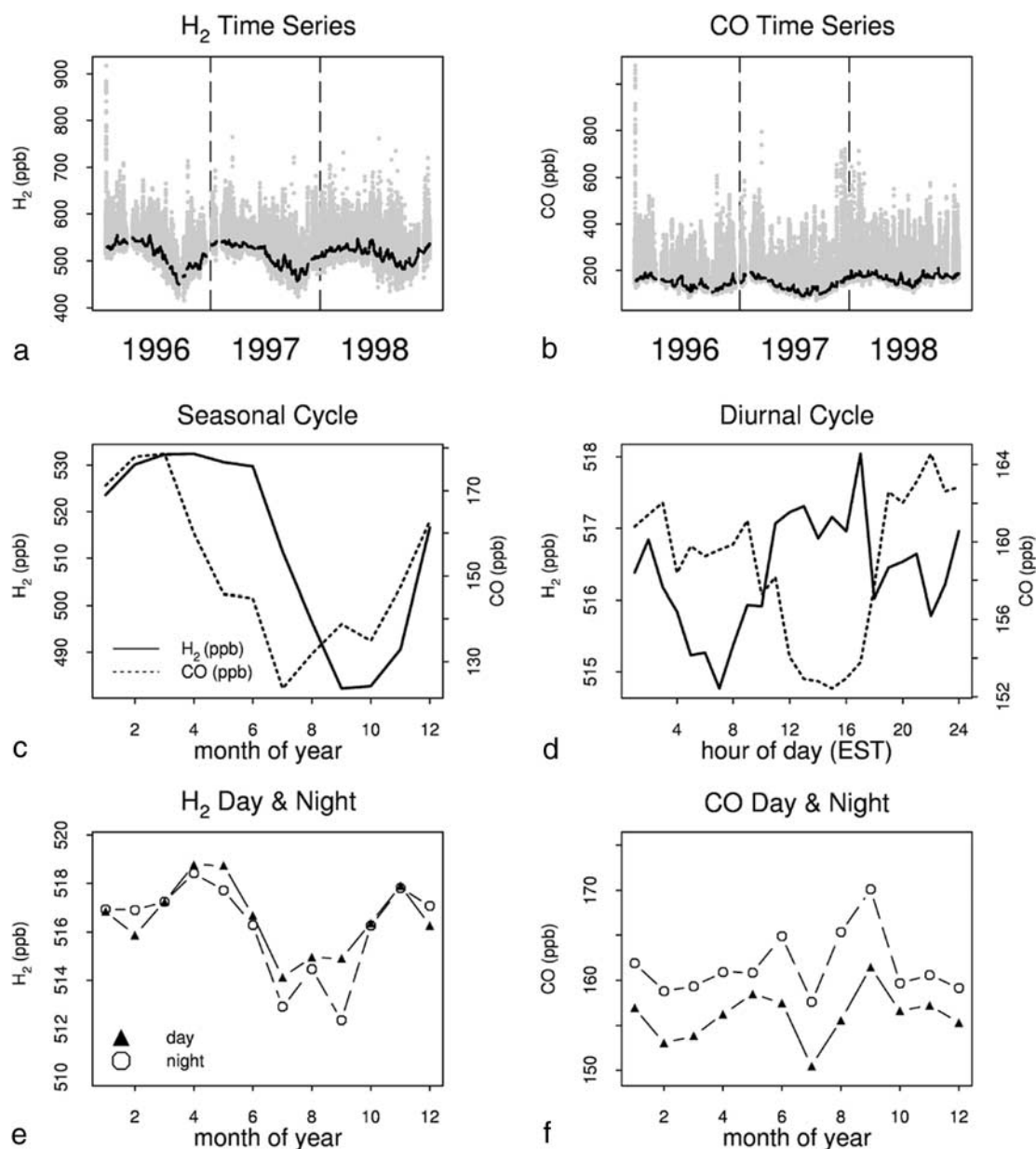
Figure 2. (a and b) Time series of \text{H}_2 and CO at Harvard Forest over the years 1996–1998. The background signals (black line) are based on a running quantile of 0.2 and an interval of 10 days. Pollution plumes are clearly evident above the background. (c) The mean background seasonal cycles of \text{H}_2 and CO. (d) \text{H}_2 and CO diurnal cycles. Each hourly point represents the median concentration for all three years of data. (e and f) Median daytime (6 am to 6 pm) \text{H}_2 concentrations exceed their nighttime (6 pm to 6 am) counterparts throughout the year, except during the winter months when the soils are frozen. For CO, daytime oxidation by OH suppresses daytime values below nighttime ones throughout the year.
