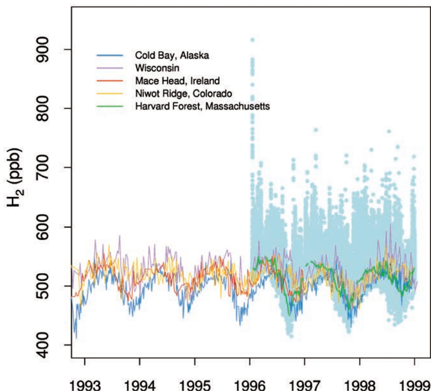
Figure 1. Comparison of background Harvard Forest hydrogen levels (green line) to those measured at Northern Hemisphere remote stations of NOAA/CMDL (as retrieved from the NOAA/CMDL web site: ftp://ftp.cmdl.noaa.gov/ccg/h2/flask ). The full H_2 data set measured by FACTS at Harvard Forest is presented.
