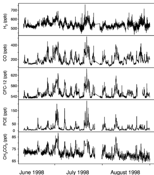
Figure 3. Pollution events from the southwest during Summer 1998 for the species H_2 , CO, CFC-12, PCE, and CH_3CCl_3 . The signals track each other closely.
