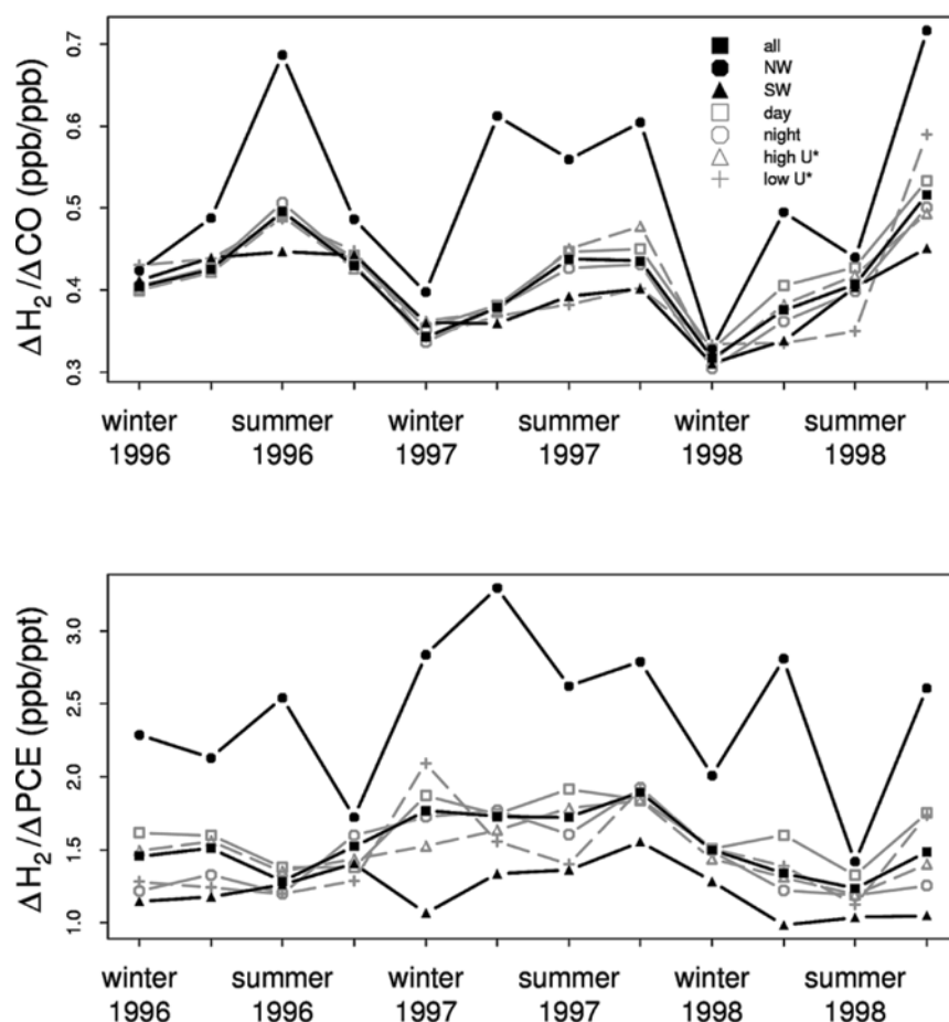
Figure 4. \Delta\text{H}_2/\Delta\text{CO} (ppb/ppb) and \Delta\text{H}_2/\Delta\text{PCE} (ppb/ppt) orthogonal distance regressions for each season and for seven cases of: all data; northwest winds only (NW); southwest winds only (SW); day (6 am to 6 pm); night (6 pm to 6 am); high U^* ( >0.2 m/s); and low U^* ( <0.2 m/s).
