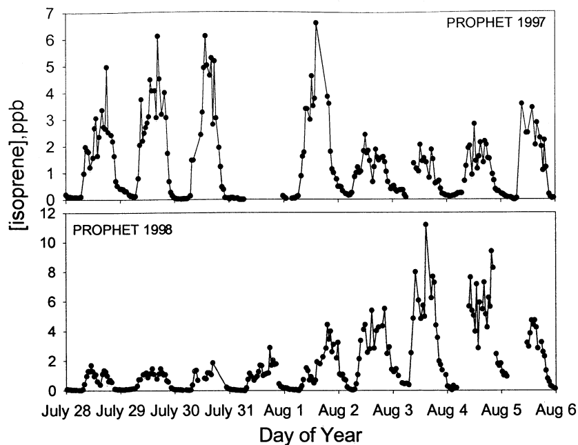
Figure 3. PROPHET 1997 and 1998 isoprene profiles.
