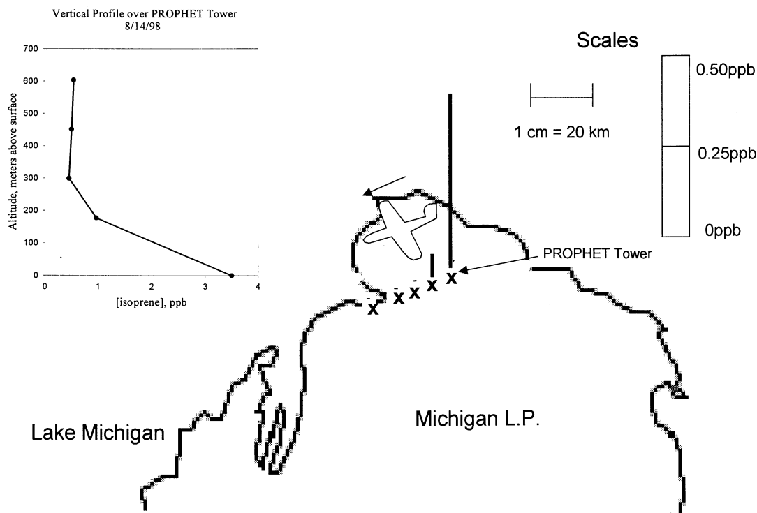
Figure 5. Isoprene Flight Data; vertical and horizontal profiles (450 m agl) for August 14, 1998, 1600 EDT. The flight began at the PROPHET tower and proceeded into the wind (WSW 3.2 m/s) out over Lake Michigan. Each sample collection point is indicated with a cross and the height of the bar over the cross represents the isoprene concentration in the sample.
