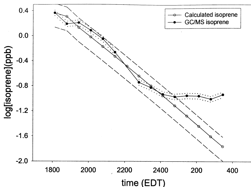
Figure 7. Calculated and observed isoprene for August 7, 1998.
