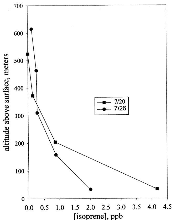
Figure 8. Evening (~1800 EDT) vertical profiles for Pellston, Michigan, July 1998.
