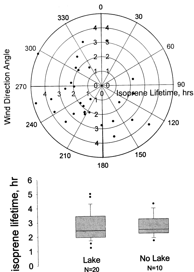
Figure 6. (top) Isoprene lifetime versus wind direction mode. (bottom) Isoprene lifetimes plotted as a function of lake influence. Boxes represent 25th and 75th percentiles, error bars represent 5th and 95th percentiles, and individual points are outliers.
