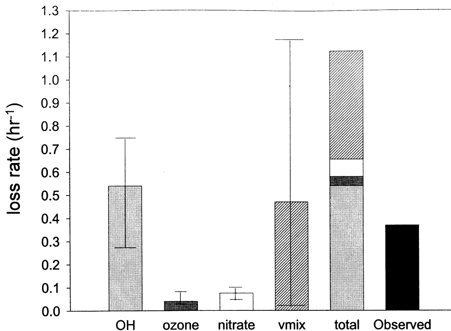
Figure 9. Contributions to isoprene loss rate. Error bars represent the calculated or estimated uncertainties for each stack.
