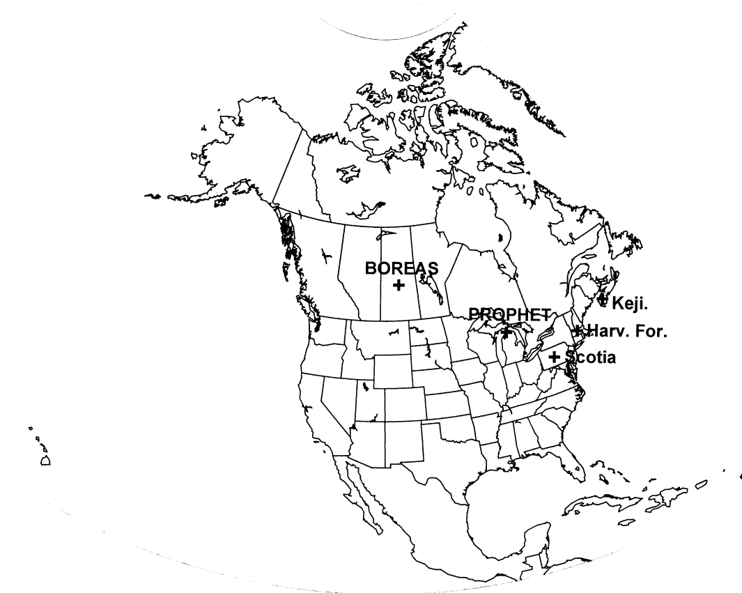
Figure 1. Map of field campaign locations. Included are inland sites, such as BOREAS, Scotia, and Harvard Forest, in addition to sites upwind of -lakes or oceans, such as Kejimikujik and PROPHET.
