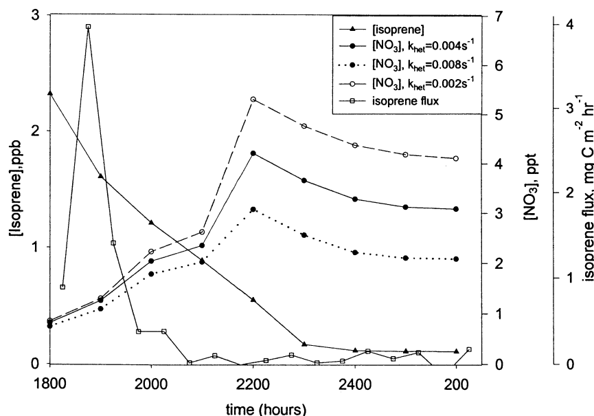
Figure 4. Isoprene concentration, isoprene flux, and simulated [NO 3 ] versus time for August 7, 1998. Nitrate radical concentrations were simulated from the average midnight values of O 3 , NO, NO 2 , HCHO, CH 3 CHO, \alpha -pinene, and \beta -pinene.
