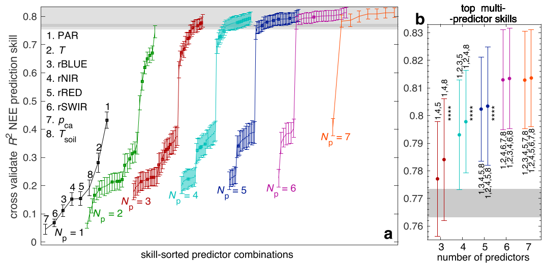
Figure 1. Cross-validated NEE predictive skill of various artificial neural network(6,5,4) models. We explore such models with one predictor ( N_p = 1 , leftmost black curve, with predictors identified numerically along the curve and by name on the upper left), and N_p = 2-7 (other color curves). For each N_p value, we consider all possible predictor combinations, and plot the sorted mean NEE predictive skill of each set \pm standard deviations calculated for each model over a set of 100 Monte Carlo realizations, each 10^3 data points long, drawn at random from the validation set that was not used in the optimization. Models (predictor combinations) whose predictors are all members of VPRM's six predictors are highlighted with square symbols. In both panels, dark gray shading around R^2 \approx 0.77 shows the cross-validated R^2 skill of the VPRM nonlinear regression estimated by the same randomization. In (a), light gray shading shows the R^2 range of panel (b), which highlights the NEE predictive skill ranges of the two most skillful predictor combinations with three to seven predictors. Panel (b) asterisks indicate the significance of the R^2 difference from the left neighbor, with one to four asterisks denoting p < 0.05 , 0.01, 0.005, and 0.001. NEE = net ecosystem exchange; PAR = photosynthetically active radiation; NIR = near infrared; SWIR = shortwave infrared.
