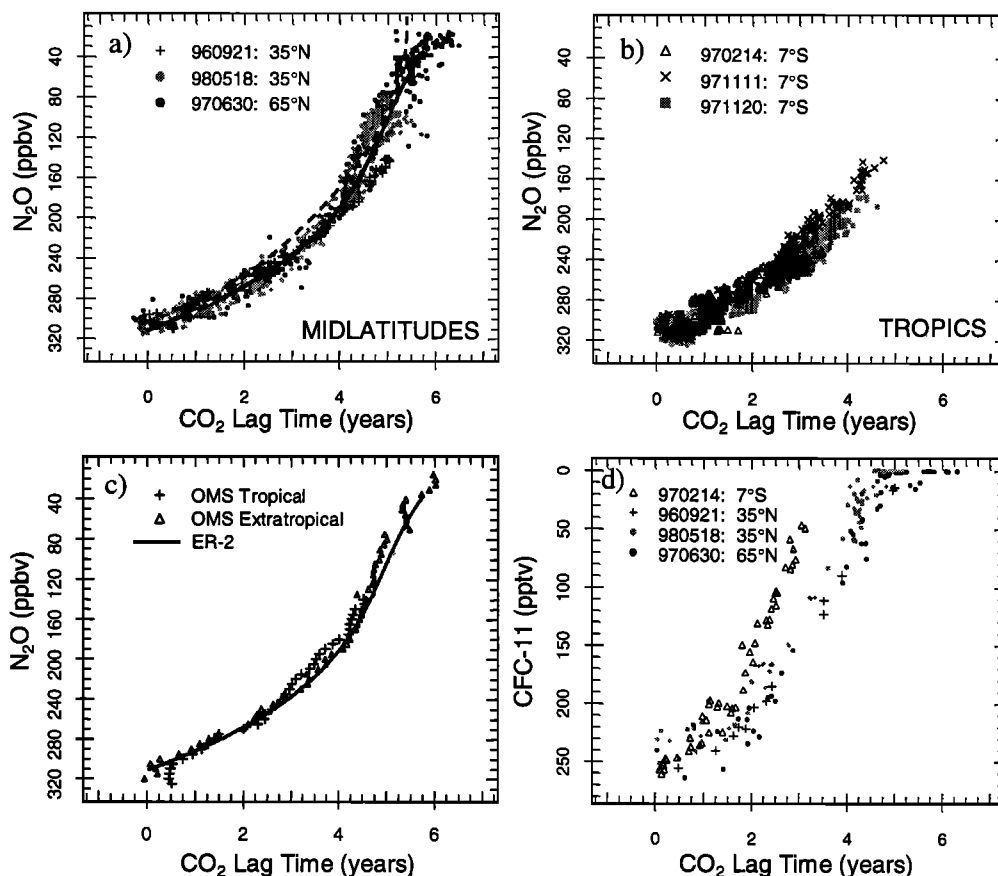
Figure 8. \Gamma_{LAG} versus N 2 O for each of the (a) extratropical and (b) tropical OMS balloon flights; (c) average relationships between \Gamma_{LAG} and N 2 O for the extratropical and tropical flights. N 2 O data are from ALIAS-II, except for the November 11, 1997, flight where data are from the Argus instrument. N 2 O mixing ratios have been normalized to the 1997 tropospheric value following Strahan et al. [1999]. The polynomial fit to the ER-2 data from Figure 3 is shown for comparison (solid line in Figures 8a and 8c) along with the midlatitude “reference relationship” given by Strunk et al. [2000] (dashed line in Figure 8a). (d) \Gamma_{LAG} versus CFC-11 for the OMS flights.
