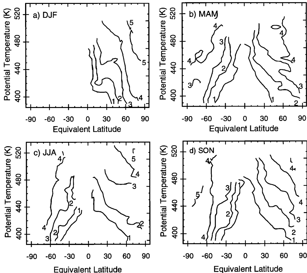
Figure 7. Climatology of \Gamma obtained by mapping the polynomial \Gamma :N 2 O relationship shown in Figure 3a onto the N 2 O climatology derived by Strahan et al. [1999] from in situ measurements of N 2 O from the NASA ER-2 aircraft. Note that the N 2 O data are normalized to 1997 levels as described in the section 2.
