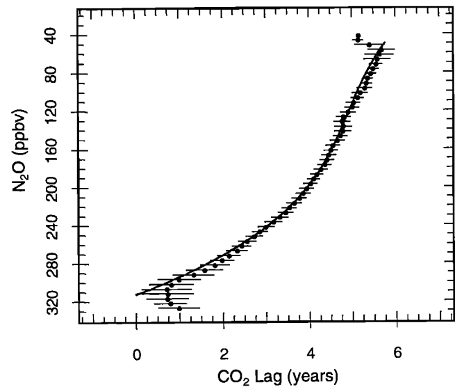
Figure 3. Average \Gamma_{LAG} (from (2)) versus N 2 O from the entire ER-2 data set, spanning latitudes from 70°S to the North Pole with data in all seasons except Southern Hemisphere summer. N 2 O measurements are from the ATLAS instrument and have been normalized to the 1997 tropospheric value following Strahan et al. [1999]. The solid circles represent the median value of \Gamma_{LAG} in overlapping 10 ppbv bins of N 2 O. The error bars represent 1 standard deviation. The solid curve is a polynomial fit excluding values corresponding to N 2 O < 50 ppbv given by \Gamma_{LAG}(N_2O) = 0.0581(313 - N_2O) - 0.000254(313 - N_2O)^2 + 4.41 \times 10^{-7}(313 - N_2O)^3 , where 313 ppbv is the average tropospheric N 2 O mixing ratio for the period from 1992 to 1998. The open triangles represent mean ages for the midlatitude lower stratosphere from the empirical age spectrum analysis of Andrews et al. [2001], referred to as \Gamma_{SPEC} in this paper.
