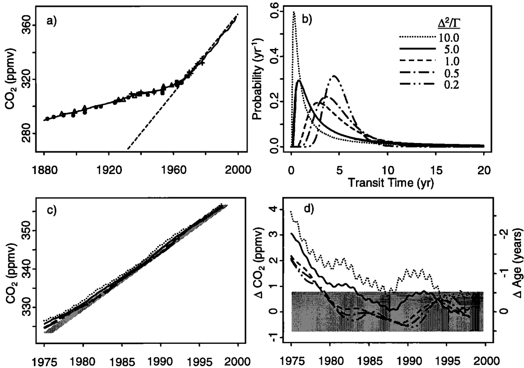
Figure 2. (a) The deseasonalized CO 2 boundary condition since 1880, derived for three periods as described below. Period 1974–1999, from surface data for Mauna Loa, HI and American Samoa, as described in the caption for Figure 1; period 1958–1974, based on annual mean CO 2 mixing ratios measured at Mauna Loa from 1958 to 1974 scaled to match the later years using overlapping data acquired from 1974 to 1993 [Keeling and Whorf, 1994]; period 1880–1958, using data from Antarctic Law Dome ice cores [Etheridge et al. , 1996]. Symbols denote cores DE08 (triangles), DE08-2 (pluses), and DSS (solid circles). The dashed line is a linear fit to the boundary condition for 1980 to 1998 (same as the solid line in Figure 1a). (b) Test age spectra with mean age = 5 years. Spectra have the functional form of the analytic solution to the Green’s function for the 1-D advection-diffusion equation [Hall and Plumb, 1994; Andrews et al. , 1999, 2001], which has been shown to fit age spectra from more complicated models of the stratosphere reasonably well. (c) CO 2 time series generated by convolving the boundary condition shown in Figure 2a plus a seasonally varying component (as in Figure 1a) with the age spectra shown in Figure 2b. (d) CO 2 time series from Figure 2c detrended by subtracting the linear fit to the CO 2 boundary condition from 1980 to 1998 (dashed line in Figure 2a) delayed by 5 years. This represents the differences between CO 2 evolution predicted using the long-term trend in Figure 2a and that which would occur if the CO 2 growth rate were constant at 1.47 ppmv yr -1 with no seasonal cycle.
