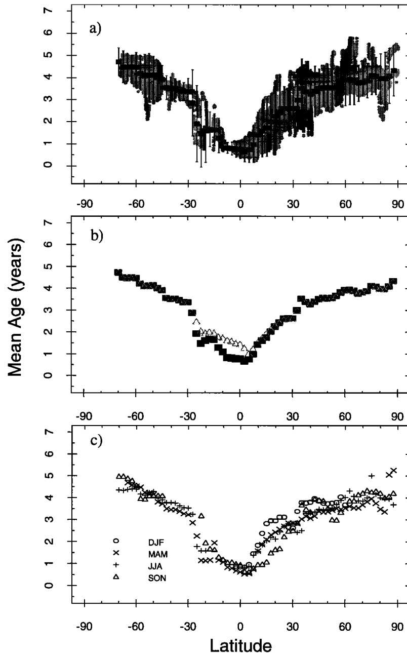
Figure 6. (a) Variation with latitude of \Gamma from all ER-2 observations of CO 2 at 20 ± 0.5 km from 1992 to 1998. Shaded symbols represent 10-s average data from each flight. Solid symbols with error bars ( \pm 2\sigma ) represent the average \Gamma in overlapping 5° latitude bins. (b) Comparison of average latitudinal variation of \Gamma (calculated using (3), solid circles) and \Gamma_{LAG} (calculated using (2), open triangles) at 20 ± 0.5 km from 1992 to 1998. (c) Seasonal variation of \Gamma as a function of latitude.
