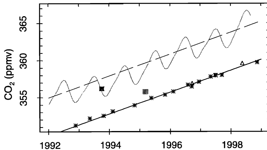
Figure 11. Average CO 2 mixing ratio corresponding to 215 ppbv N 2 O as measured on the ER-2 for 1992 - 1998 (asterisks), on the midlatitude OMS balloon flights, and as reported by Harnisch et al. [1998] at ~20 km (simultaneous measurements of N 2 O were 215 ± 5 ppbv); symbols for the balloon data are the same as in Figure 10. The shaded line and the dashed line are the same as in Figure 10. The solid line has the same slope as the linear fit to the boundary condition but with a delay of 3.5 years.
