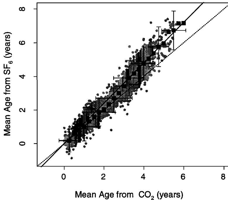
Figure 9. Scatterplot of mean ages derived from SF 6 and CO 2 observations from the NASA ER-2. The dotted line is the 1:1 line, and the solid line is the 1.2:1 line. Shaded symbols represent the 10-s flight data. Solid squares with error bars ( \pm 2\sigma ) denote the average SF 6 age in overlapping 0.5 year intervals of CO 2 age.
