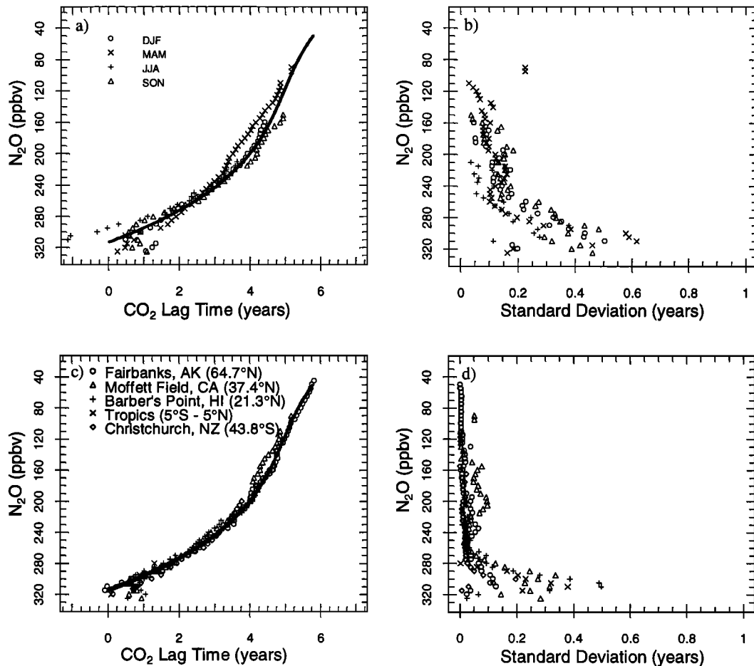
Figure 4. (a) \Gamma_{LAG} (from (2)) versus N 2 O for measurements from the NASA ER-2 aircraft within 2.5° of NASA Ames Research Center in Moffett Field, California (37.4°N), for each of the four seasons. N 2 O mixing ratios have been normalized to the 1997 tropospheric value following Strahan et al. [1999]. Each symbol represents the median mean age in a 10 ppbv N 2 O interval. DJF, December-January-February; MAM, March-April-May; JJA, June-July-August; SON, September-October-November. (b) The corresponding standard deviations. (c) Average \Gamma_{LAG} as a function of N 2 O for measurements from the NASA ER-2 aircraft within 2.5° of airfields where the airplane was based during SPADE, ASHOE/MAESA, STRAT, and POLARIS and for measurements obtained within 5° of the equator. Each symbol represents the median mean age in a 10 ppbv N 2 O interval. (d) The corresponding standard deviations. See text for discussion of sampling at each location. The curve shown in Figures 4a and 4c is the cubic fit to mean ages from the entire ER-2 data set, as shown in Figure 3.
