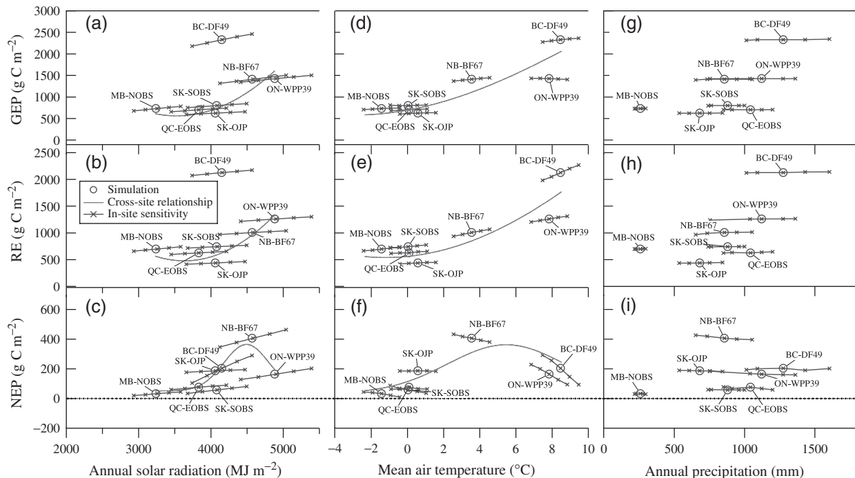
Fig. 5 Cross-site comparison of simulated annual GEP, RE and NEP, and in-site sensitivity to total solar radiation (a–c), mean air temperature (d–f) and total precipitation (g–i), at all the seven conifer forest sites across Canada. The sensitivity analysis at each forest site was conducted by changing incident solar radiation at \pm 5\% and \pm 10\% , air temperature at \pm 0.5 and \pm 1.0 ^{\circ}\text{C} and precipitation at \pm 10\% and \pm 20\% of observed values, respectively, and one at a time while the rest unchanged.
