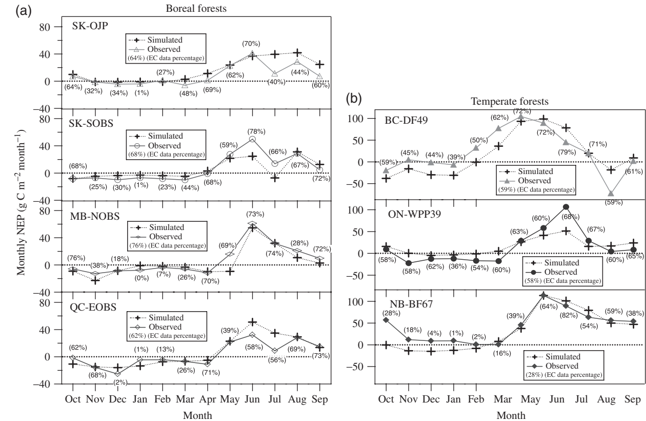
Fig. 4 Comparison of CN-CLASS simulated and measured (gap-filled) monthly NEP at all the seven conifer forest sites across Canada. Note that the percentage of nongap-filled measured data is shown for each month.
