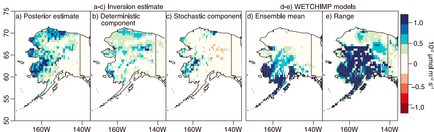
Figure 4. (a) The \text{CH}_4 fluxes estimated by the GIM, averaged over all time periods (May–October 2012–2014). (b and c) The individual components of the posterior flux estimate; the sum of these two panels equals the posterior estimate in Figure 4a. (d and e) The mean and range, respectively, of seven process-based \text{CH}_4 fluxes estimates from the recent WETCHIMP model comparison project [Melton et al. , 2013].
