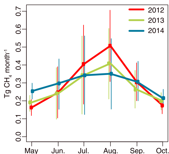
Figure 3. Estimated \text{CH}_4 budgets for Alaska by month for 2012–2014. The vertical lines show the associated uncertainties (one standard deviation).
