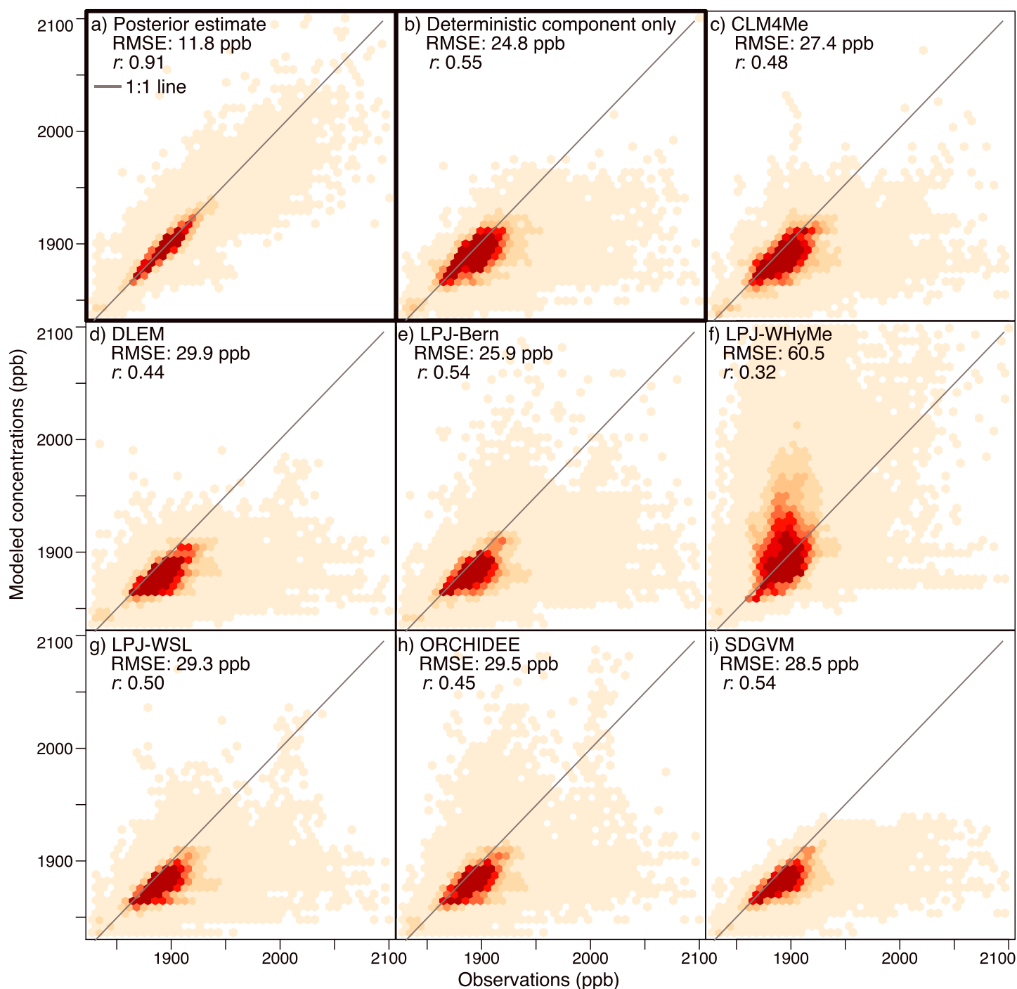
Figure 5. This plot compares atmospheric \text{CH}_4 concentrations modeled with PWRP-STILT against \text{CH}_4 observations from the CARVE aircraft and CRV tower. We model \text{CH}_4 concentrations using a number of flux estimates: (a) the posterior estimate from the GIM, (b) the deterministic component from the GIM, and (c–i) process-based flux estimates from the WETCHIMP comparison study [Melton et al. , 2013]. Darker colors indicate a higher density of points in each scatterplot. Note that the process-based estimates are more comparable to the deterministic model than the posterior estimate; the process-based estimates and deterministic model rely on auxiliary variables or environmental driver data sets. In contrast, the posterior estimate also includes fluxes that do not map on to any auxiliary variable.
