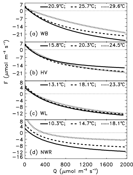
Figure 1. Ecosystem light response curves for each AmeriFlux site for three different temperature regimes. The regression curves were obtained by fitting the data using equation (1). More negative numbers mean greater carbon uptake from atmosphere by ecosystems.
