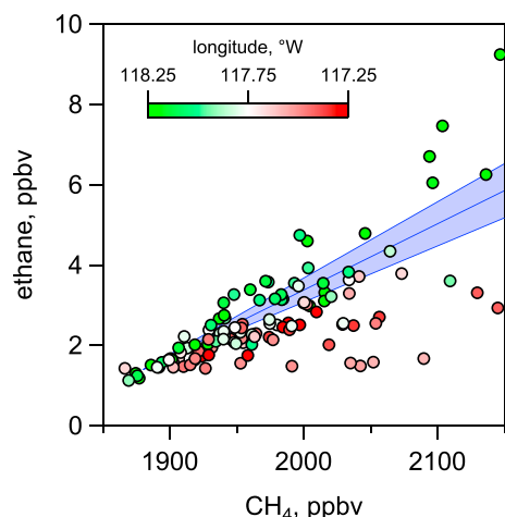
Figure 4. Scatter plot of ethane versus \text{CH}_4 from the NOAA P-3 data in the L.A. basin. Data points are colored by longitude to show the different distributions of ethane to \text{CH}_4 in the eastern (red) and western (green) parts of the basin. The blue line represents the slope of 1.65 \pm 0.25 % used by Wennberg et al. [2012] to represent the estimated ethane/ \text{CH}_4 ratio of pipeline-quality dry natural gas from the Southern California Gas Company's pipelines.
