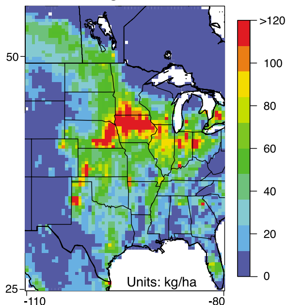
Figure 9. An estimate of annual fertilizer use taken from Potter et al. [2010]. The a posteriori N 2 O fluxes from both the geostatistical and Bayesian inversions are strongly similar to the spatial distribution of nitrogen fertilizer. Potter et al. [2010] estimate manure application for 2007 and synthetic fertilizer for 2000.
