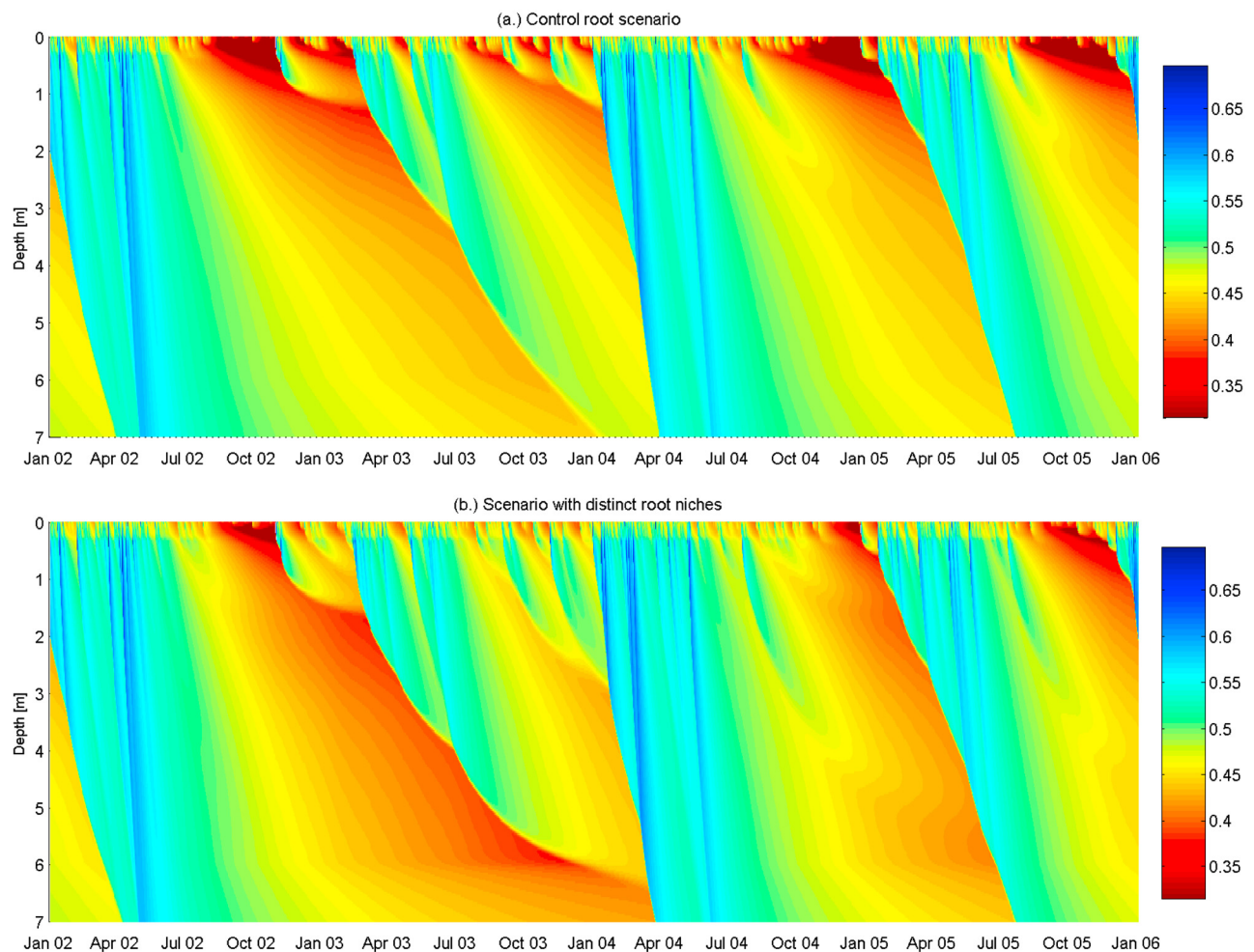
Figure 5. The temporal evolution of soil moisture profile for two root scenarios corresponding to the maximum root depth Z_{Roots} . (a) Simulation results for the control root scenario are illustrated, which exhibits the same fractional distribution of roots for all tree types (Table 3). (b) Simulation results for the scenario with distinct root niches are shown. The scenario assumes that trees of the upper canopy level contain a higher fraction of roots at deeper locations, while trees of the bottom-canopy layer contain higher fraction of roots at shallower soil layers (Table 3). The “CO” soil type was used.
