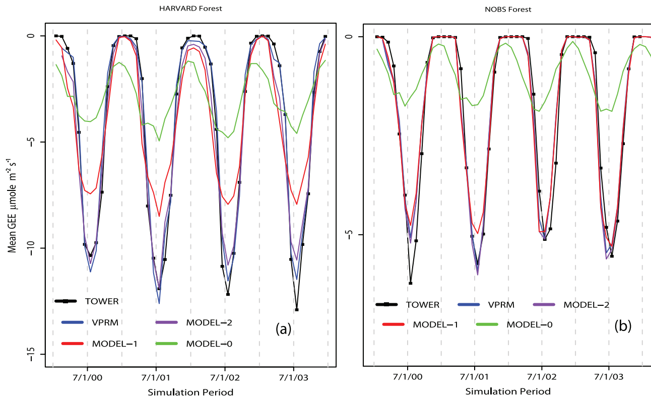
Figure 7. A comparison between GEE ( \mu\text{mole m}^{-2} \text{s}^{-1} ) obtained by fitting VPRM, MODEL-2, MODEL-1, and MODEL-0 to tower data from 2000 to 2003 at Harvard Forest (a) and NOBS/BOREAS (b). VPRM incorporates EVI, P_{\text{scale}} , and W_{\text{scale}} (driven by satellite data), plus T_{\text{scale}} driven by meteorological data. MODEL-2 drops LSWI factors ( P_{\text{scale}} and W_{\text{scale}} ), MODEL-1 drops all satellite
