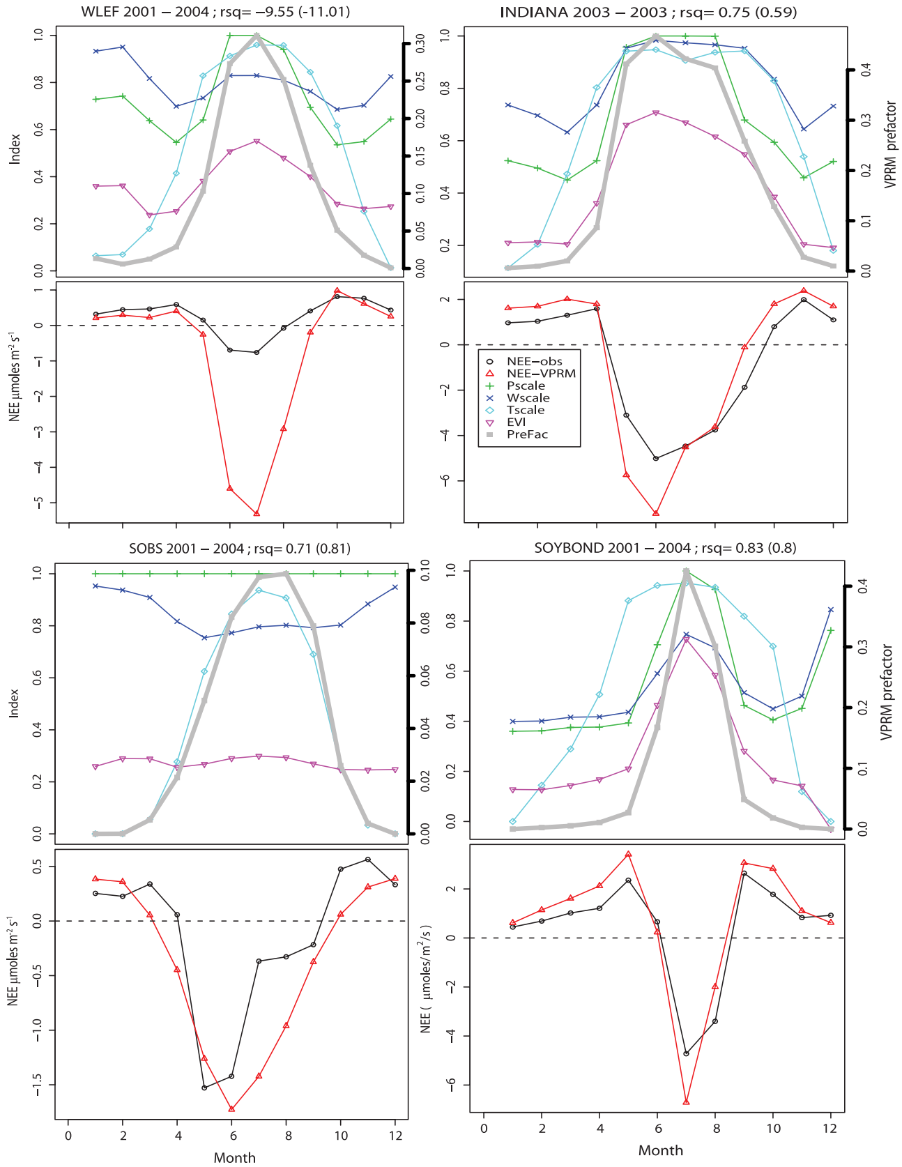
Figure 5. A comparison of the seasonal dynamics of model and observed NEE, as in Figure 3, but at validation sites (no adjustment of VPRM parameters).
