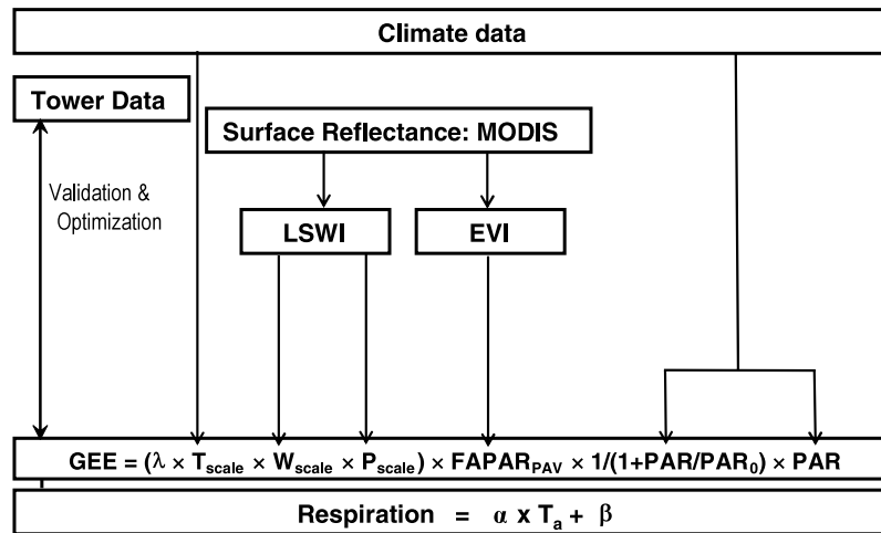
Figure 1. Schematic diagram of the Vegetation Photosynthesis Respiration Model (VPRM). EVI: Enhanced Vegetation Index; LSWI: Land Surface Water Index; FAPAR_{PAV} : the fraction of incident light absorbed by the photosynthetically active vegetation in the canopy; T_{scale} , P_{scale} , and W_{scale} : scalars for temperature, leaf phenology, and canopy water content, respectively. Gross Ecosystem Exchange (GEE) is the light-dependent part of Net Ecosystem Exchange (NEE), and Respiration (R) is the light-independent part. MODIS refers to the Moderate Resolution Imaging Spectroradiometer onboard the NASA Terra and Aqua satellites; PAR_0 , \lambda , \alpha , and \beta are the four model parameters, one set per vegetation type.
