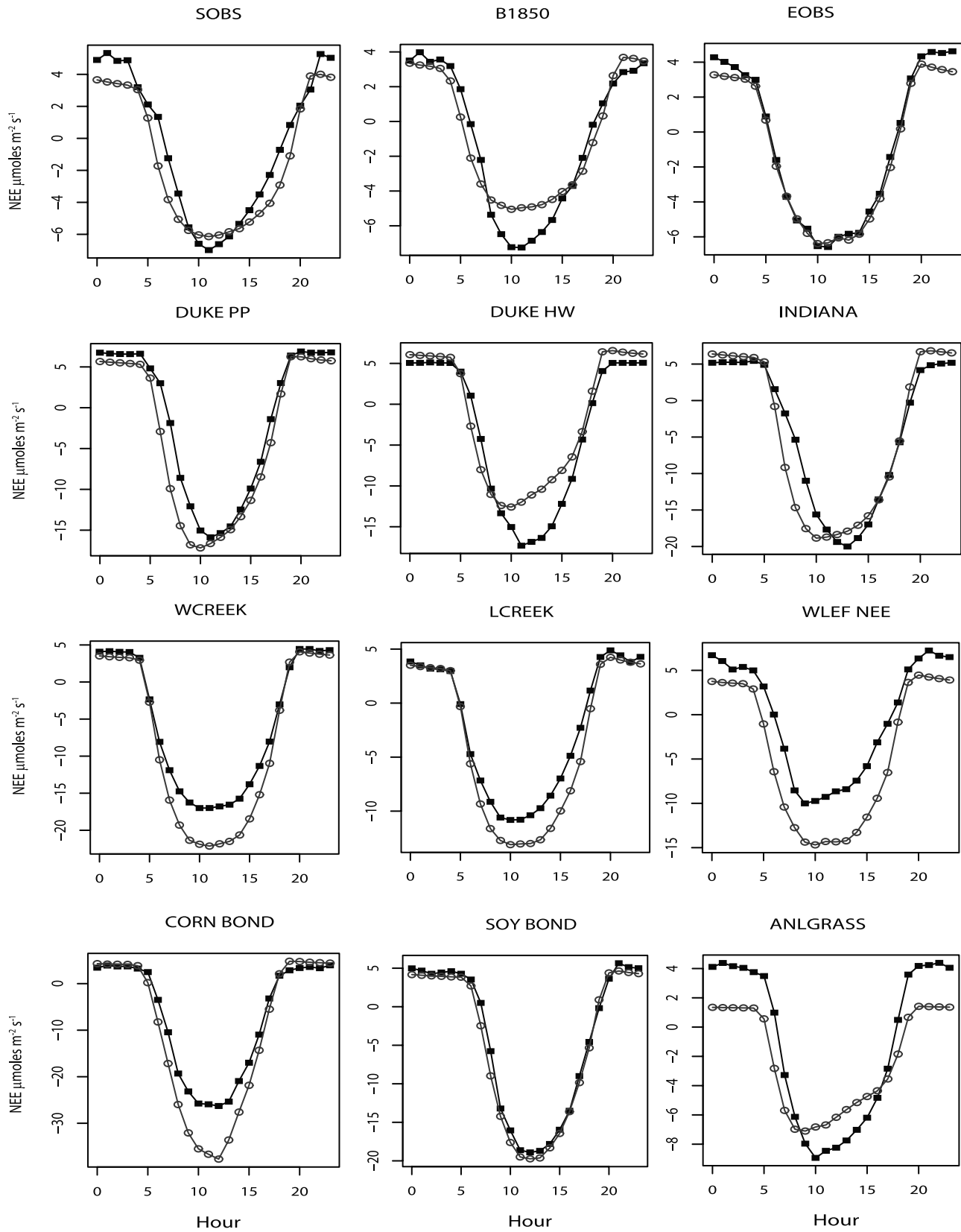
Figure 4. Comparison between the observed (solid squares) and predicted (open circles) diurnal mean NEE ( \mu\text{mole m}^{-2} \text{s}^{-1} ) over the peak photosynthetically active period, as in Figure 2b, but at validation sites without adjustment of parameters.
