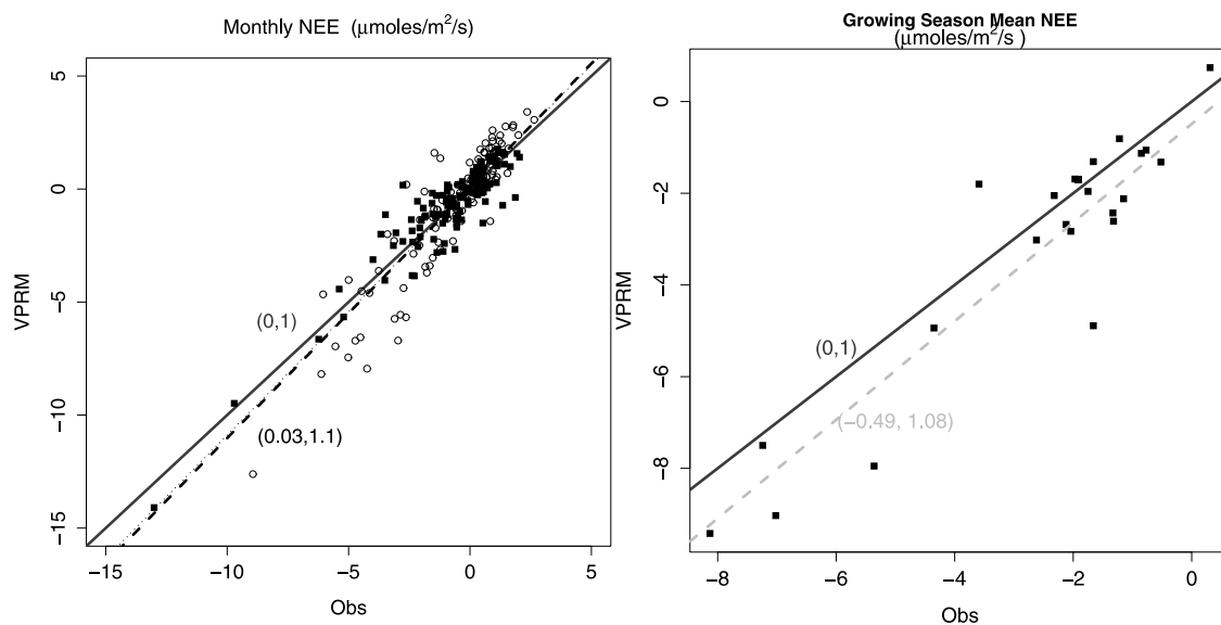
Figure 6. (left) Observed and predicted monthly mean NEE ( \mu\text{mole m}^{-2}\text{s}^{-1} ) for calibration sites (solid symbols) and validation sites (open symbols) excluding WLEF. Regression line for all sites (dotted line) is very similar to the regression for validation sites only (dashed line). (right) Mean NEE by site (except WLEF) for the growing season. Line labeled (0,1) has zero intercept and slope = 1 (“1:1 line”). Regression lines are labeled similarly.
