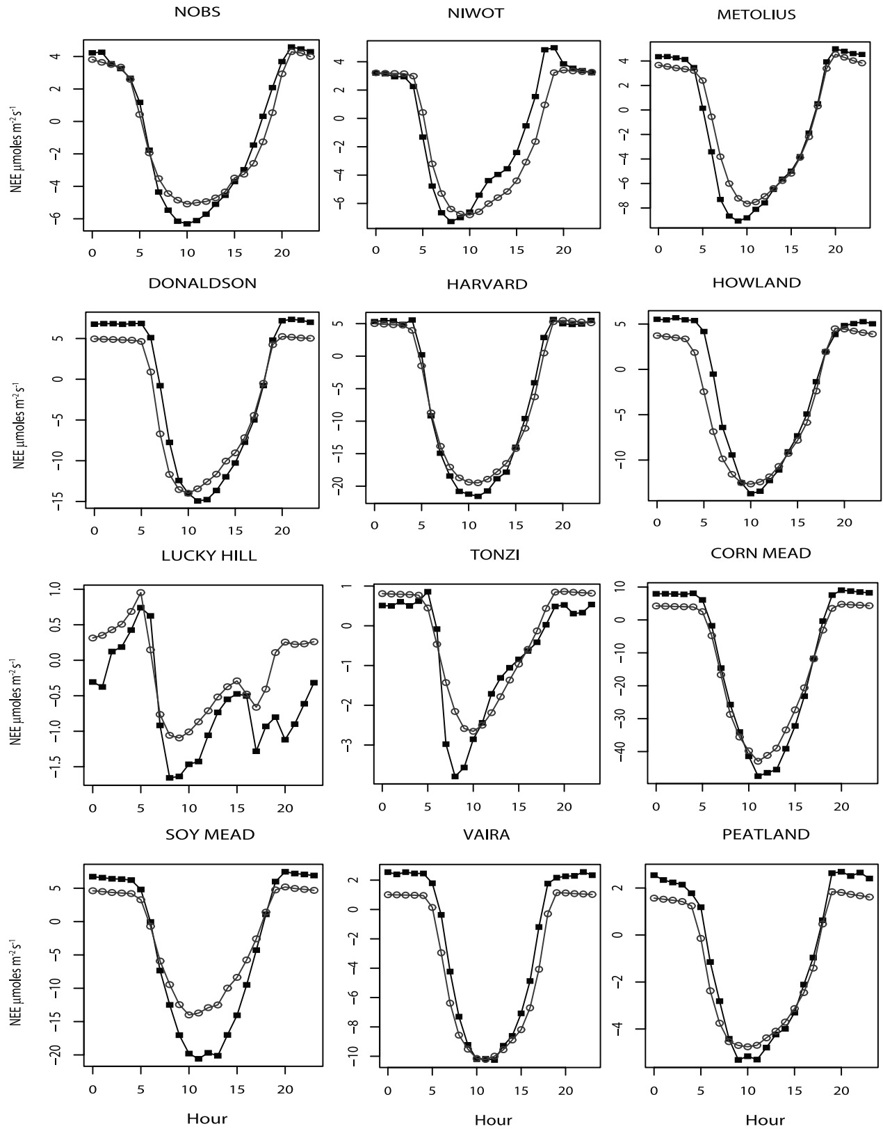
Figure 2b. A comparison between the observed (solid squares) and VPRM (open circles) mean diurnal variation of NEE ( \mu\text{mole m}^{-2} \text{s}^{-1} ) during the peak growing season at calibration sites.
