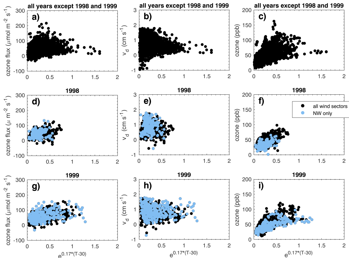
Figure 8. Hourly observed ozone fluxes (shown as positive here; \mu\text{mol O}_3/\text{m}^2/\text{s} ), deposition velocities ( v_d ; \text{cm}/\text{s} ), and concentrations (ppb) versus an exponential temperature ( T ) dependence for 9 am to 4 pm during June–September 1998 and 1999 (years where we hypothesize highly reactive biogenic volatile organic compounds play a role) versus other years at Harvard Forest. Blue indicates hours when wind comes from the NW because trees that emit highly reactive biogenic volatile organic compounds are only in the NW wind sector.
