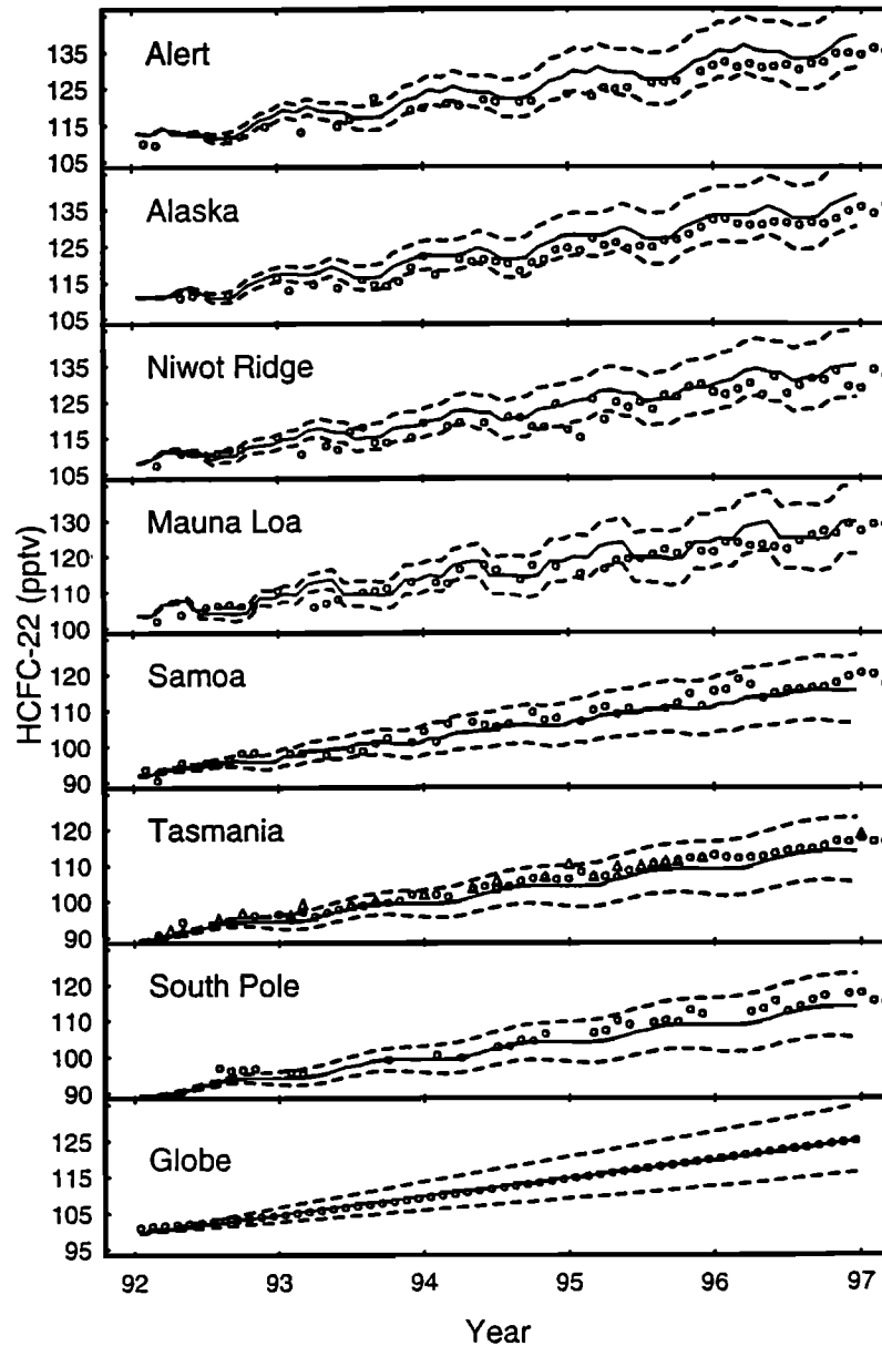
Figure 15. Observed long-term trend in HCFC-22 (circles [Montzka et al. , 1993, 1996; CMDL, 1998] and triangles [Muller et al. , 1998]) simulated using standard OH (solid lines), and with standard OH reduced and increased by 25% (dashed lines) at Alert (82°N, 63°W), Alaska (71°N, 137°W), Niwot Ridge, Colorado (40°N, 106°W), Mauna Loa (20°N, 156°W), Samoa (14°S, 171°W), Tasmania (41°S, 145°E), and South Pole (90°S, 102°E). The lowest panel (marked Globe) shows a mean of least squares polynomials of 4th degree fitted to observations and model results ((\text{Alert} + \text{Alaska} + \text{Niwot Ridge} + \text{Mauna Loa})/4 + (\text{Samoa} + \text{Tasmania} + \text{South Pole})/3)/2 .
