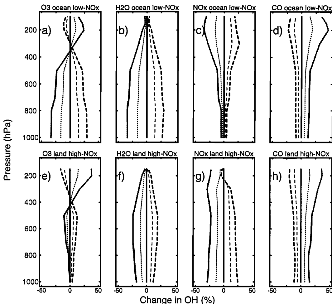
Figure 11. Change in OH (percent) in response to changes by -50\% , -25\% (dotted lines), +25\% , +50\% (dashed lines) at 15^{\circ}\text{S} over ocean in January in (a) \text{O}_3 , (b) \text{H}_2\text{O} , (c) \text{NO}_x , and (d) \text{CO} , and over land in July in response to changes in (e) \text{O}_3 , (f) \text{H}_2\text{O} , (g) \text{NO}_x , and (h) \text{CO} . Note that results for July reflect the influence of biomass burning. Thin lines correspond to \pm 25\% perturbations, and thick lines correspond to those of \pm 50\% .
