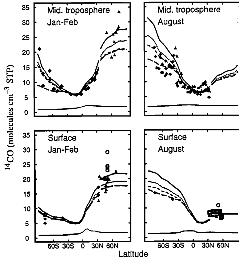
Figure 27. Concentration of ^{14}\text{CO} (molecules \text{cm}^{-3} STP) (top) at 6–7 km altitude and (bottom) at the surface (left) in January–February and (right) in August. Observations for 1990–1991 (diamonds) are from Mak et al. [1992], and for 1992 (squares) and 1993 (triangles) are from Mak et al. [1994]. Note that the cosmic source was approximately constant in 1990–1991, increasing by 8% in 1992 and additional 5% in 1993. See Figure 25 for the description of simulations and designation of line types. To facilitate a comparison with observations, model results south of 32^\circ\text{N} are shown for 1990–1991, and north of 32^\circ\text{N} for 1993. We also included observations in 1977–1978 from Volz et al. [1981] (open circles); the cosmic source for 1977–1978 was comparable to that in 1992–1993.
