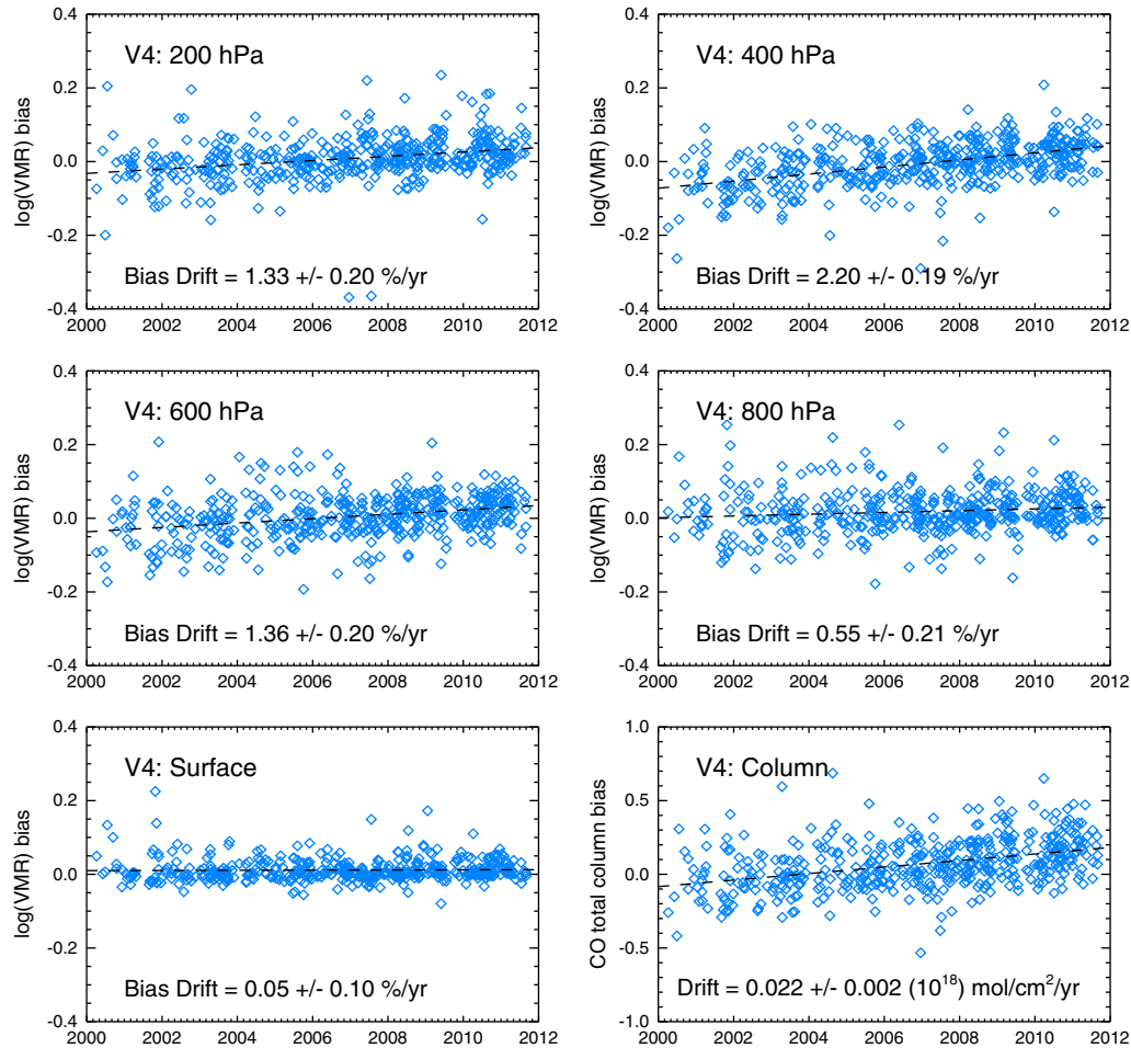
Figure 8. Time series plot showing V4 bias trends based on NOAA profiles.
